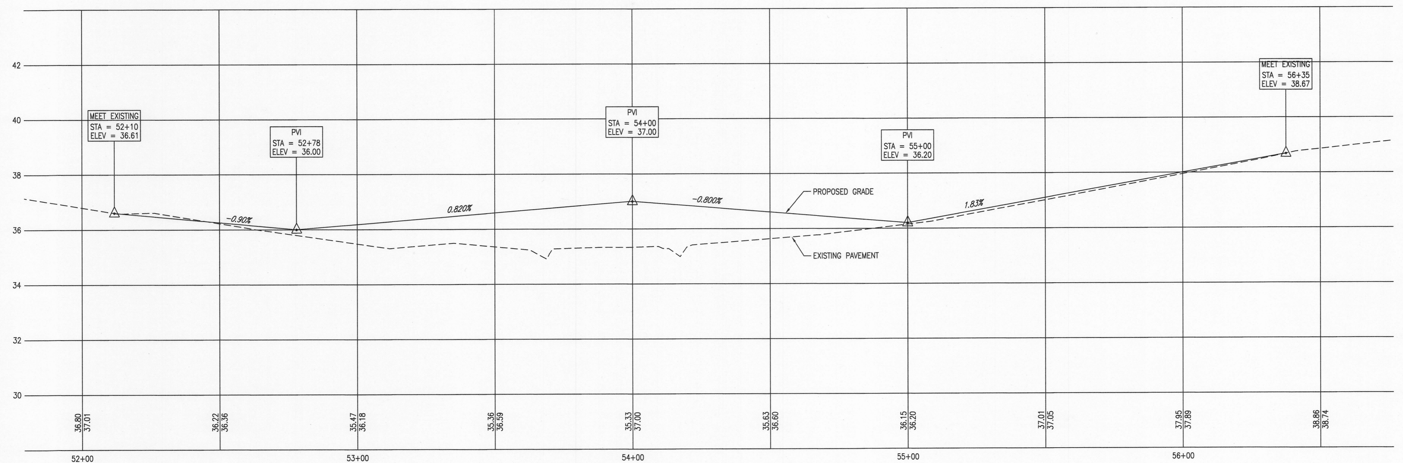
CENTERLINE PROFILE SCALE: H. 1"=20' V. 1"=2'
