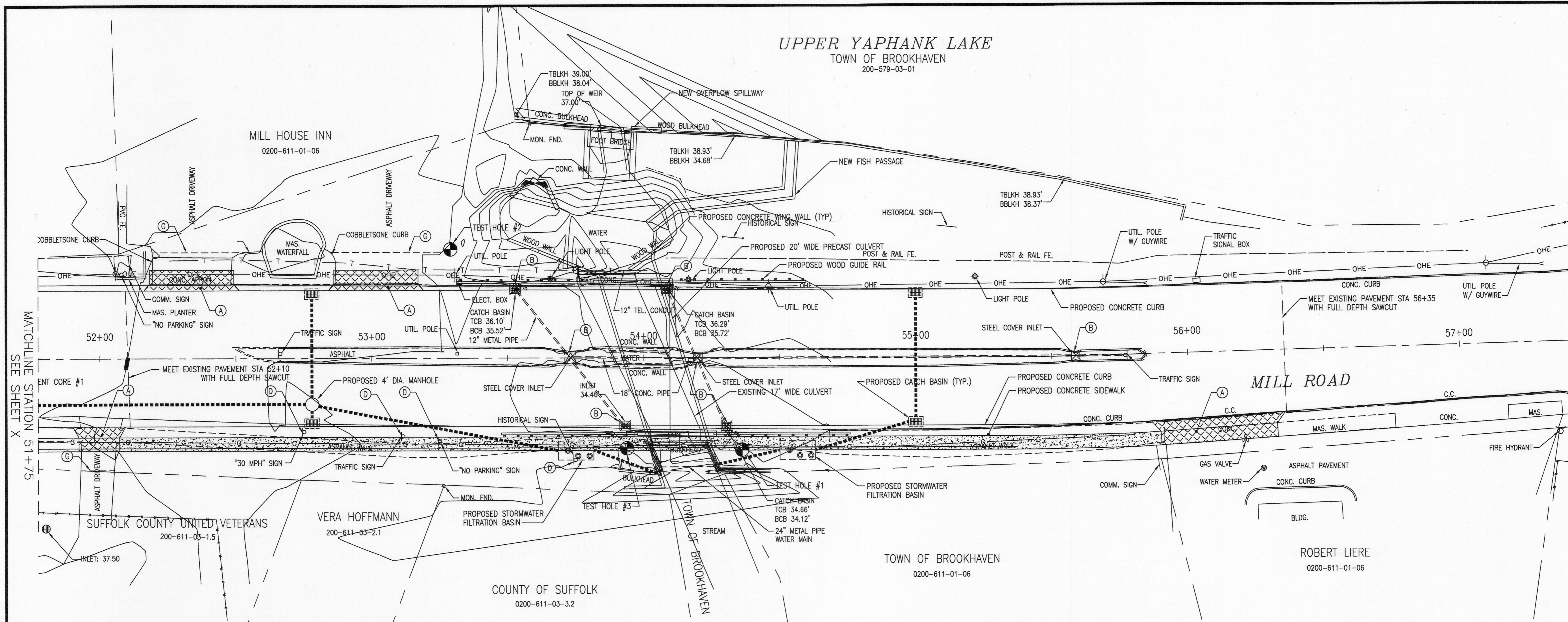
GENERAL PLAN SCALE: 1"=20'
